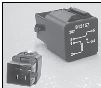
86-91 fuel pump relay
