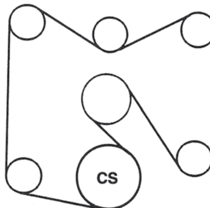
Serpentine Belt Route W/AC
